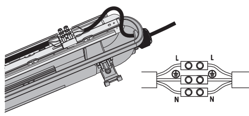
6. Connect the wires, L to L , N to N, \oplus to \oplus
