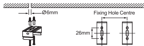
2. According to the Fixing hole centre, instal expansion bolts and screws, instal the bracket.
